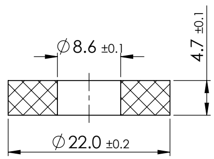
SECTION X-X
